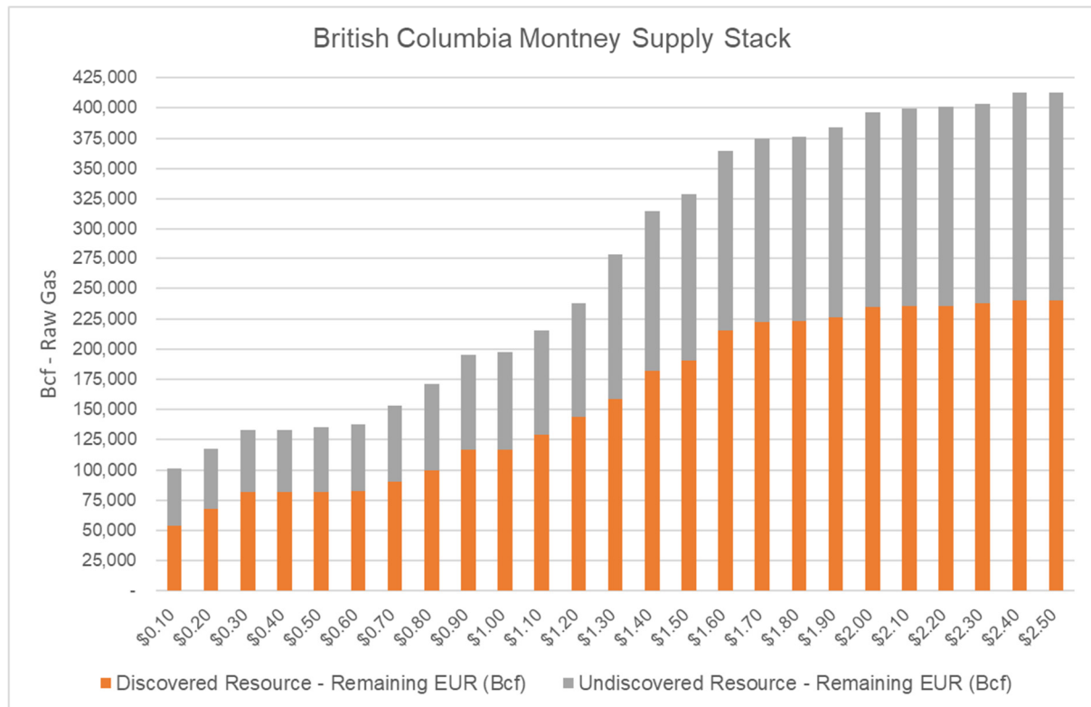
Figure 4: BC Montney Supply Stack
