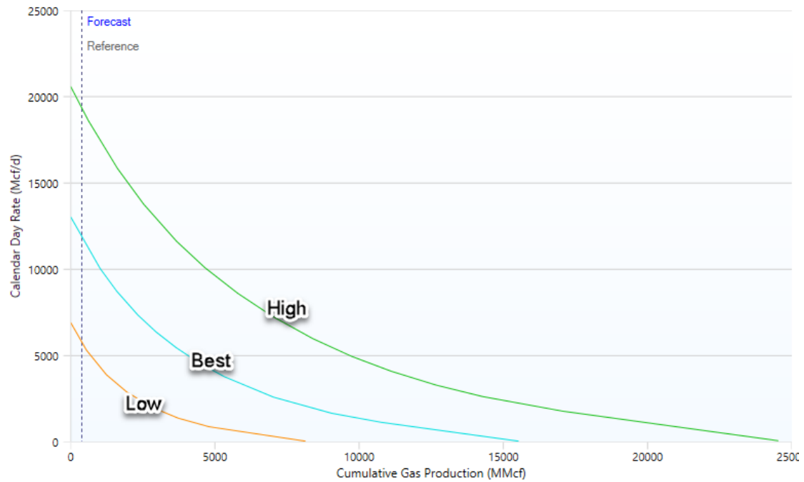
Figure 5: Area 13 Upper – Low, Best, and High Estimate Type Curves
